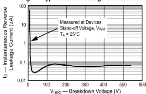
Fig. 7 – Typ. Reverse Leakage Characteristics
