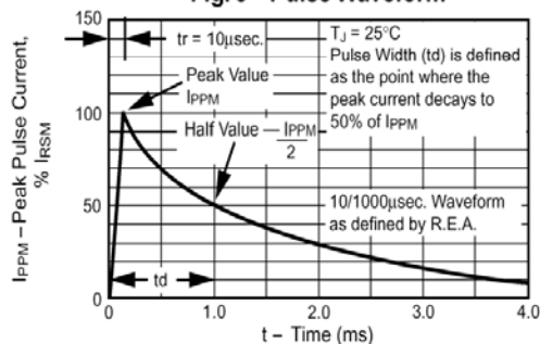
Fig. 3 – Pulse Waveform
